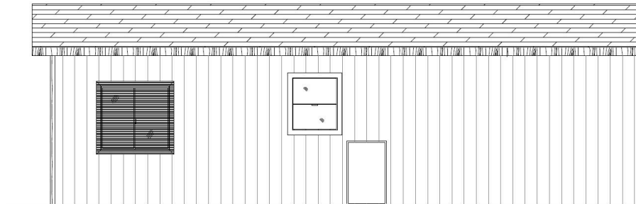
ROAD SIDE ELEVATION
