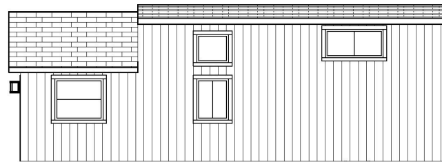
ROAD SIDE ELEVATION
