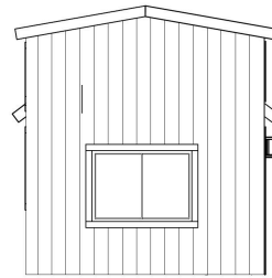
REAR END ELEVATION
